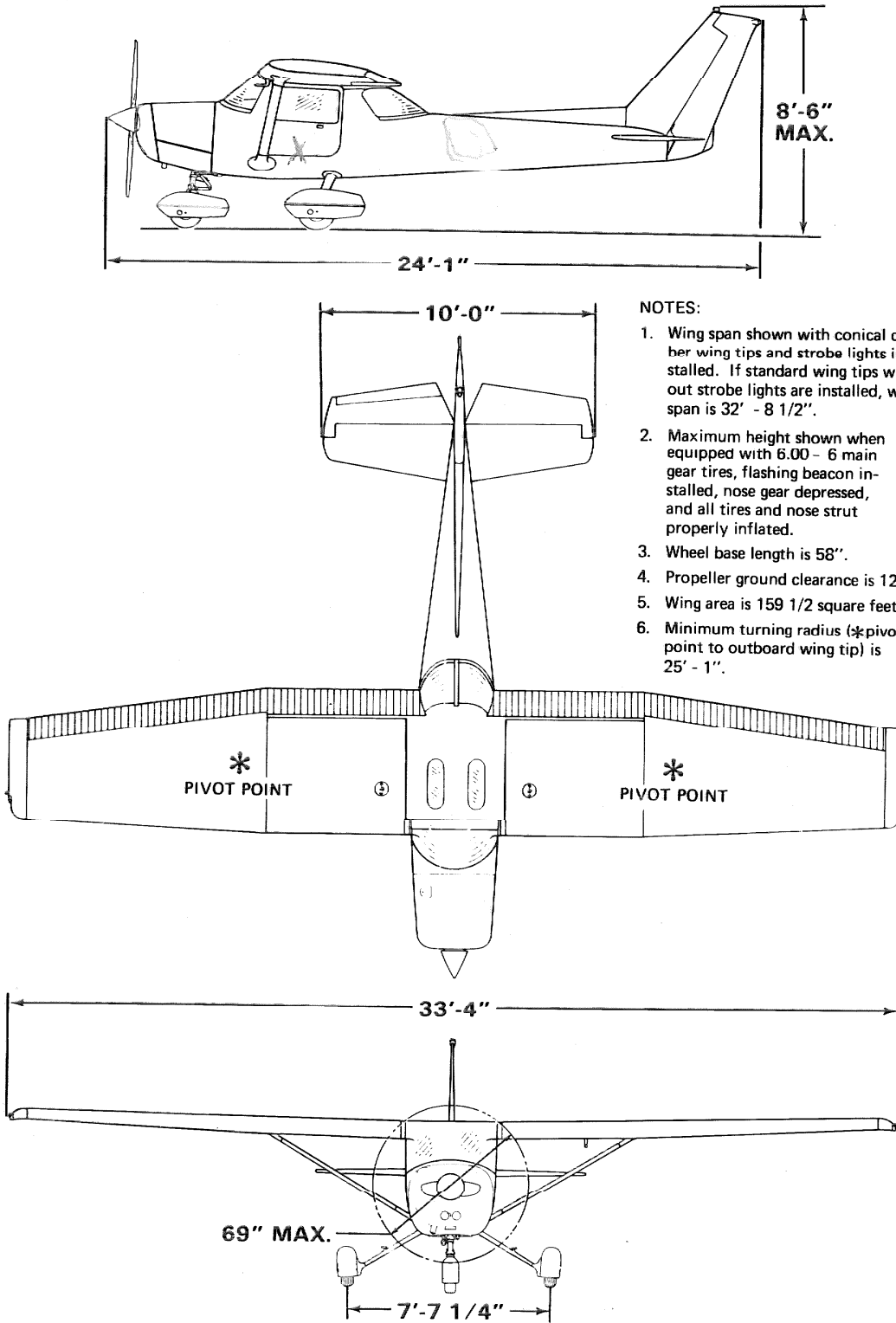
Figure 1-1. Three View
