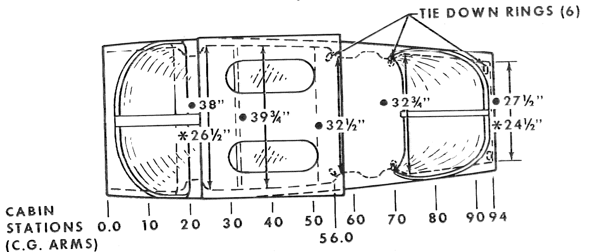
Figure 6-5. Internal Cabin Dimensions
