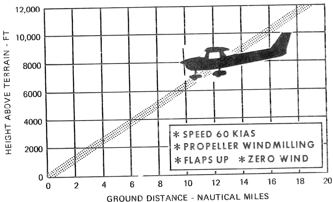
Figure 3-1. Maximum Glide
