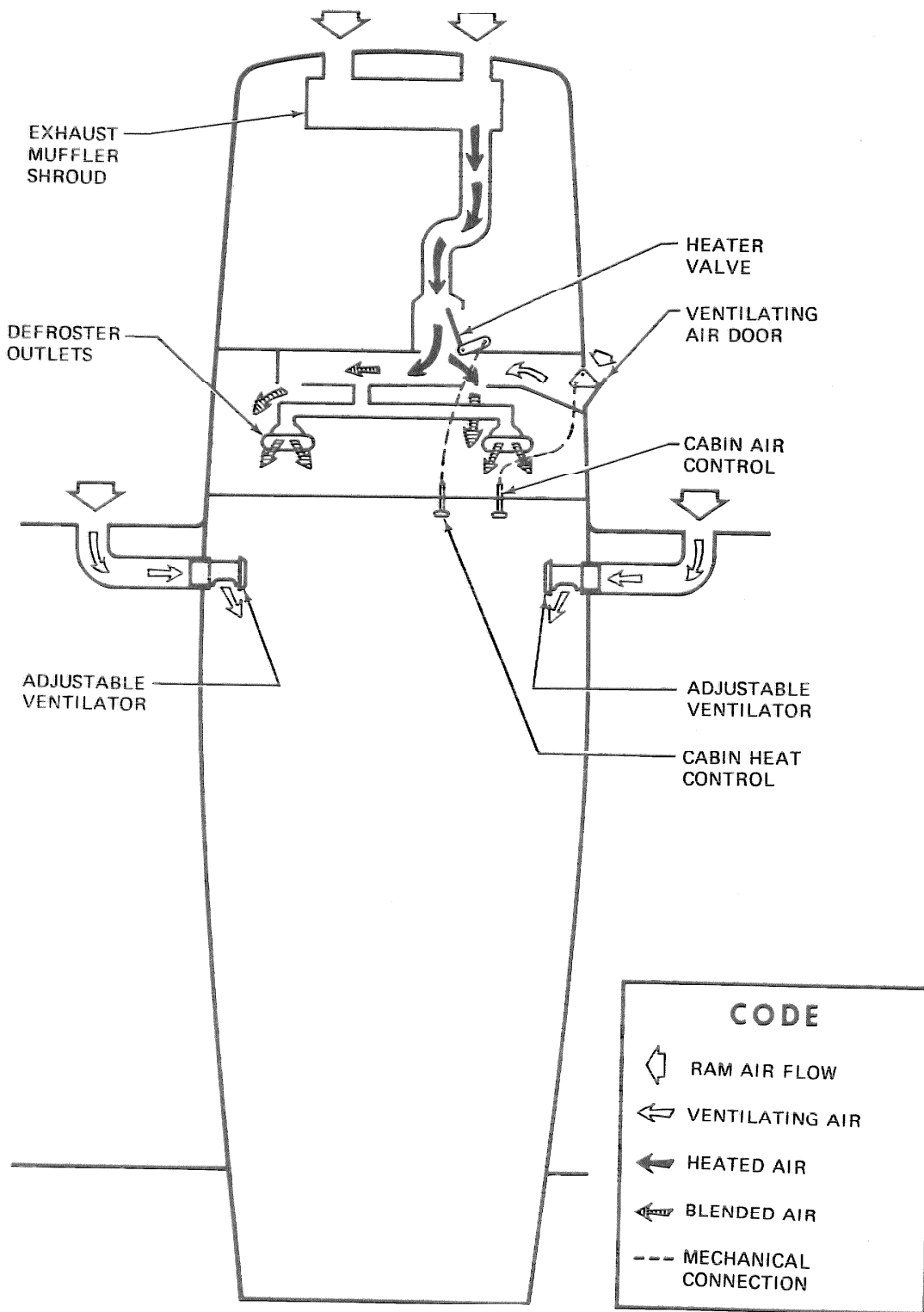
Figure 7-8. Cabin Heating, Ventilating, and Defrosting System
