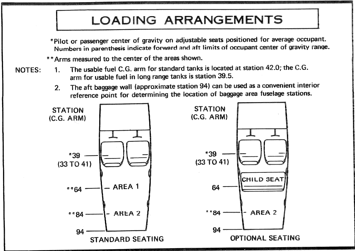
Figure 6-3. Loading Arrangements
