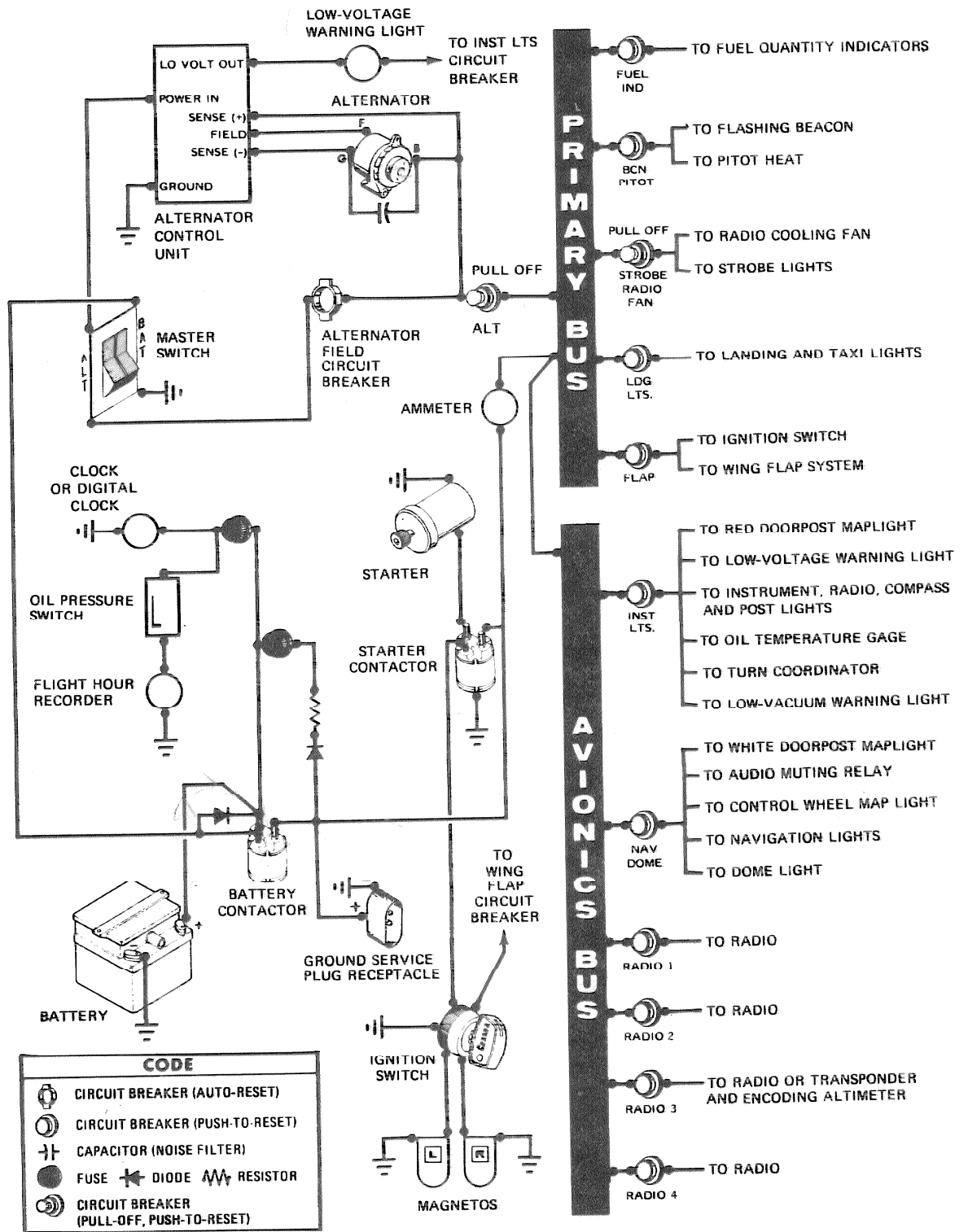
Figure 7-7. Electrical System
