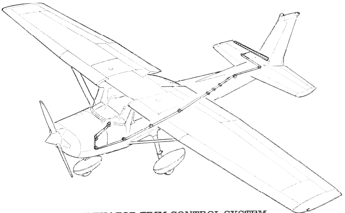
ELEVATOR TRIM CONTROL SYSTEM
