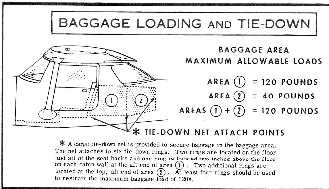
Figure 6-4. Baggage Loading and Tie-Down
