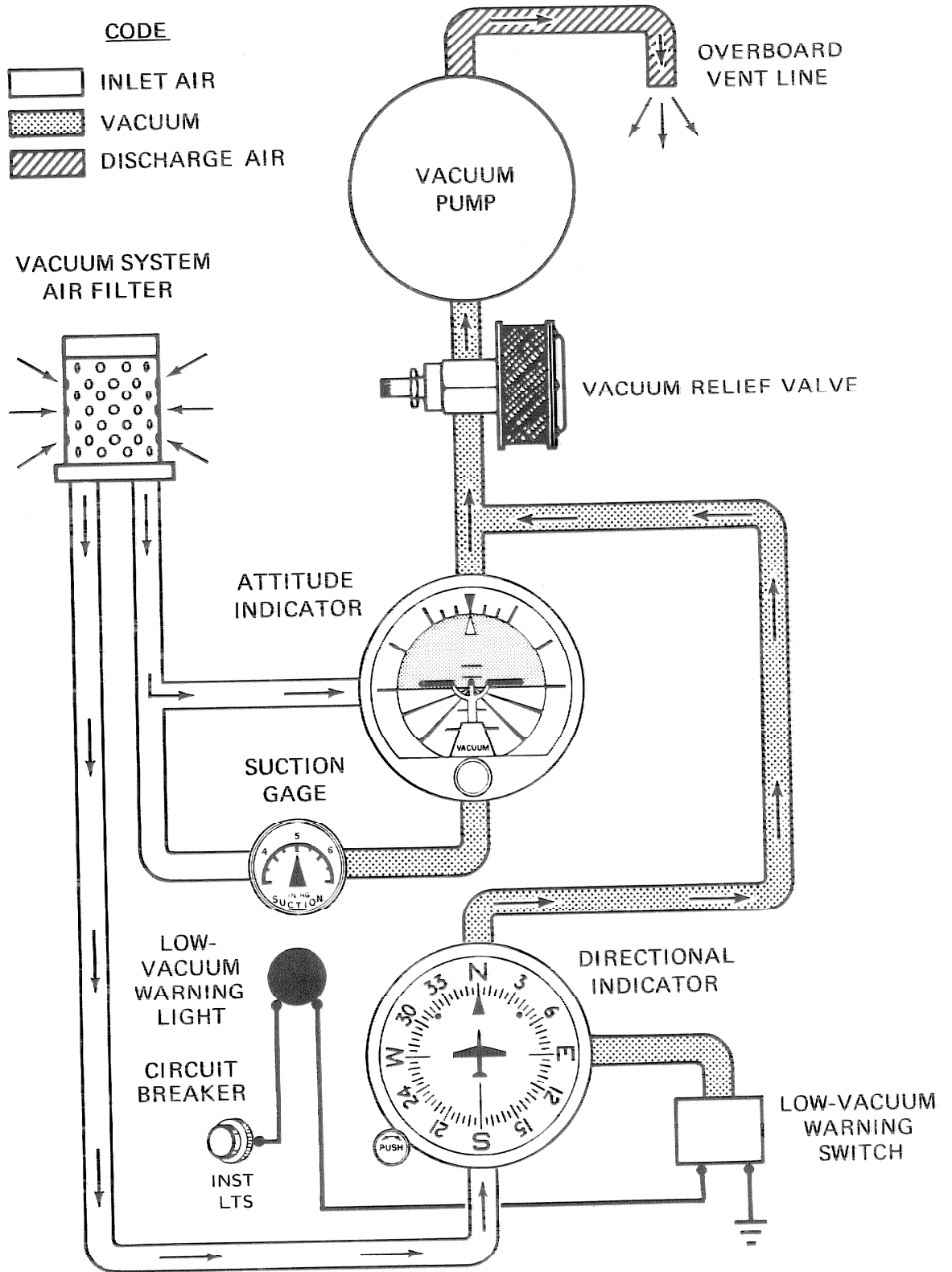
Figure 7-9. Vacuum System
